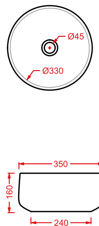
COL004 COGNAC 35 lavabo appoggio countertop washbasin
