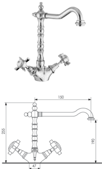
ART. S3756A MONOBLOCCO LAVABO SALTARELLO 1"1/4 LUSO (CON FLESSIBILE) WASH-BASIN UNIT WITH LUXURY 1"1/4 POP-UP WASTE (WITH FLEXIBLE)
