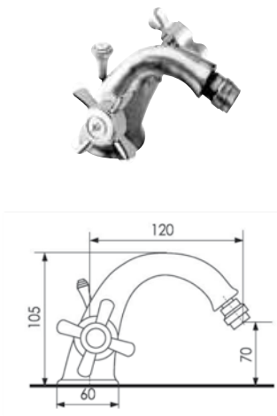
ART. S3764A MONOBLOCCO BIDET LUSO SALTARELLO 1"1/4 LUSO (CON FLESSIBILE) BIDET UNIT WITH LUXURY 1"1/4 POP-UP WASTE (WITH FLEXIBLE)
