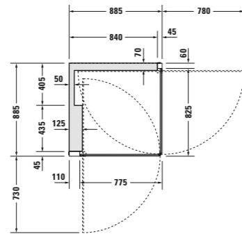
# 770008 00 0 *0 0000, 885 x 885 mm Ecke links. Corner left. Rinconera izq.
