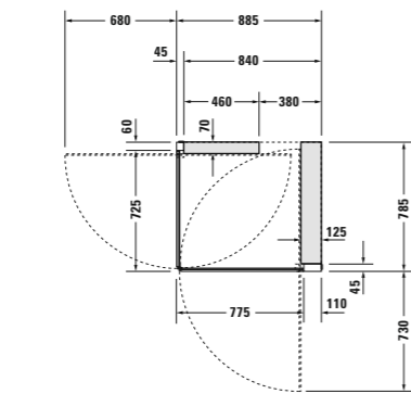
# 770010 00 0 *1 0000, 785 x 885 mm Ecke rechts. Corner right. Rinconera derecha
