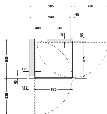
# 770012 00 0 *0 0000, 885 x 985 mm Ecke links. Corner left. Rinconera izq.
