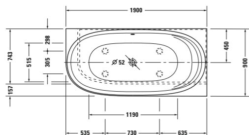
# 700363 00 00 0000, 1900 x 900 mm Ecke rechts. Corner right. Rinconera derecha
