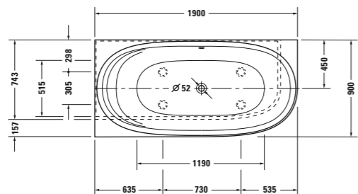
# 700362 00 00 0000, 1900 x 900 mm Ecke links. Corner left. Rinconera izq.
