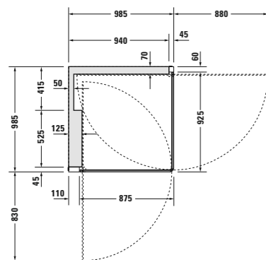
# 770009 00 0 *0 0000, 985 x 985 mm Ecke links. Corner left. Rinconera izq.
