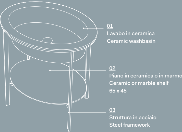
Catino Ovale 70 con cassetto \ Catino Ovale 70 with drawer - 70 x 50 x h83
