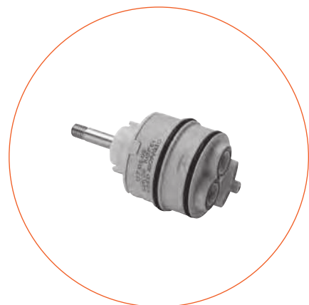
Cod. 9828 Cartuccia Ø mm. 38 38 mms. Ø cartridge per/for RIVA
