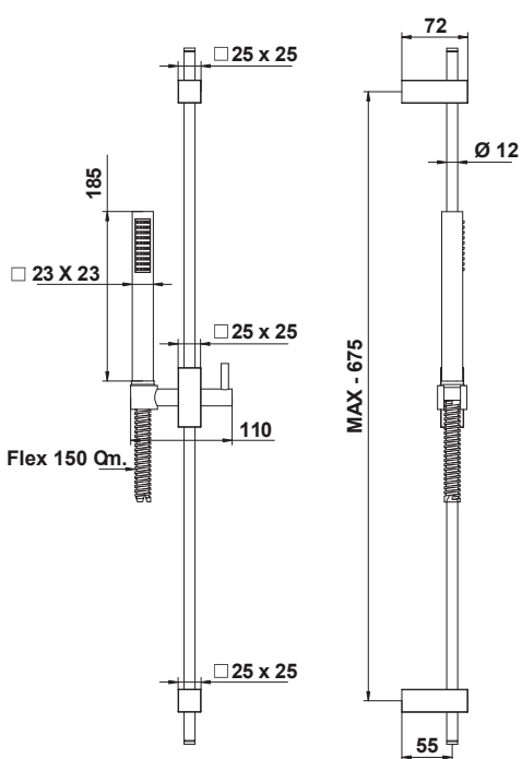
Cod. 874 Saliscendi minimalista quadro con doccetta monogetto e flessibile doppia aggraffatura mm 1500, 1/2" ff conico. Square minimalist sliding rail with single function handshower and mms 1500 double interlock hose, 1/2" ff conical.
