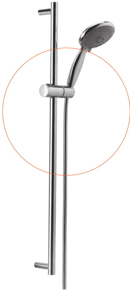
Cod. 876/N Saliscendi con doccetta a 3 getti Ø 130 mm e flessibile doppia aggraffatura mm 1500, 1/2" ff conico. Sliding rail with 3 functions Ø 130 mms handshower and mms 1500 double interlock hose, 1/2" ff conical.
